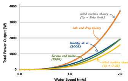
MODELLLED POWER OUTPUT AGAINST WATER SPEED
