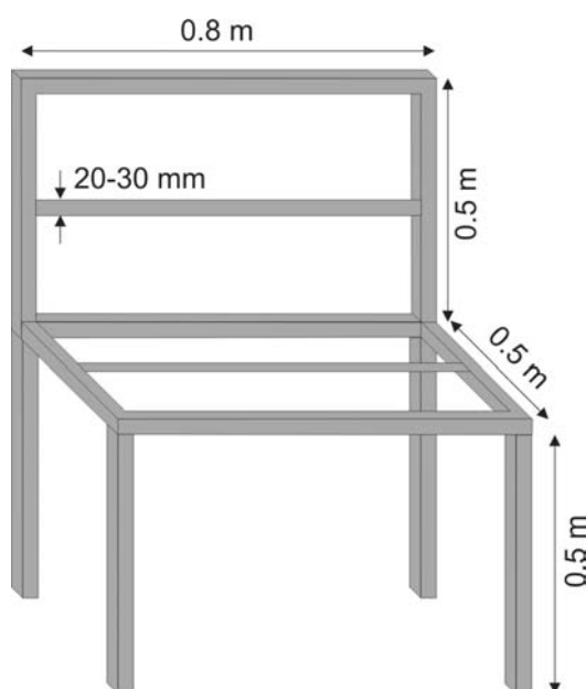
Figure 2: Chair frame
