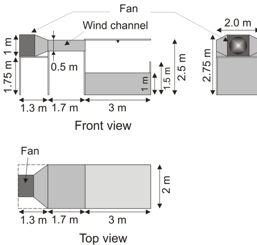
Figure 1: Balcony Mock-up
