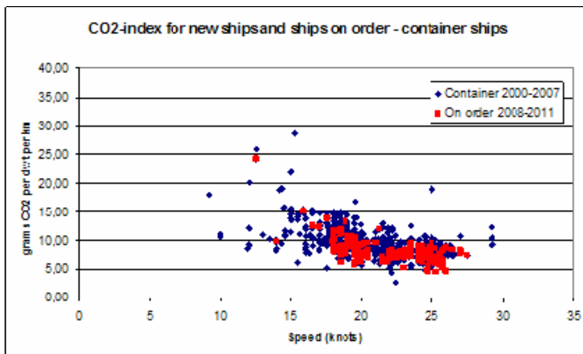
Figure 0-7: Speed vs CO 2 -index for container ships.
