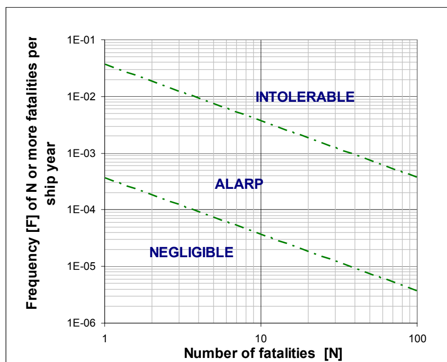
Figure 1: Acceptance criteria for societal risk of crew onboard container vessels
