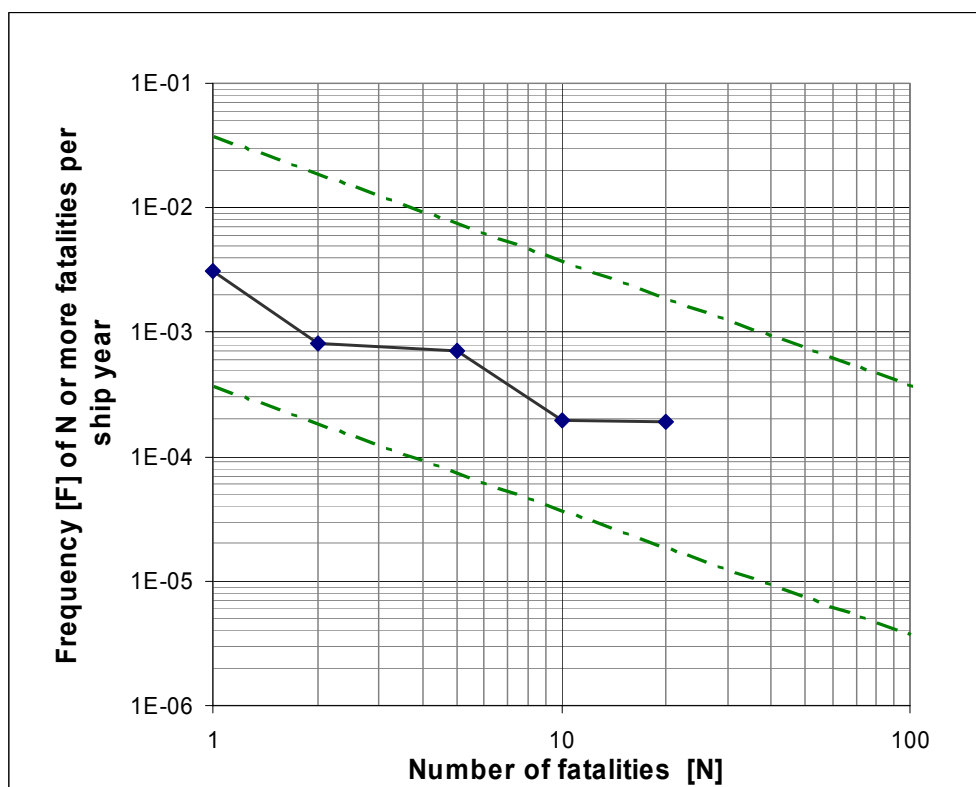
Figure 2: Societal risk of crew member onboard container vessels
