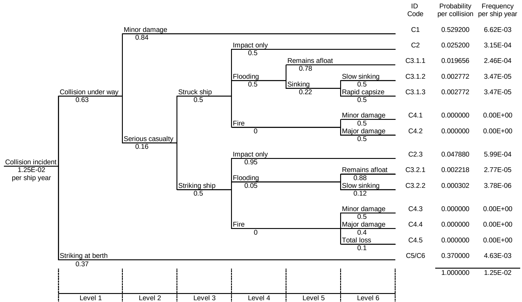
Figure 10: Generic Collision Event Tree
