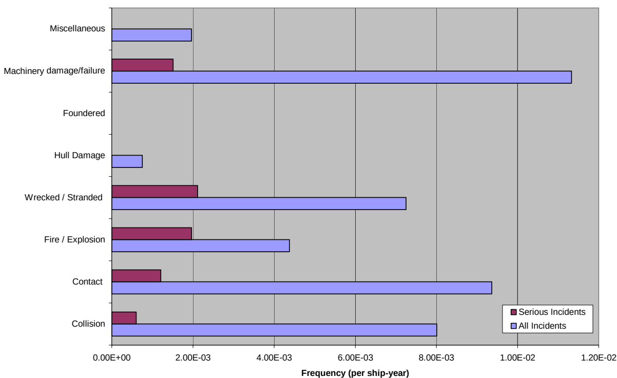
Figure 6: Frequency of Incidents, RoPax 1,000 GRT to 4,000 GRT (1994-2004)
