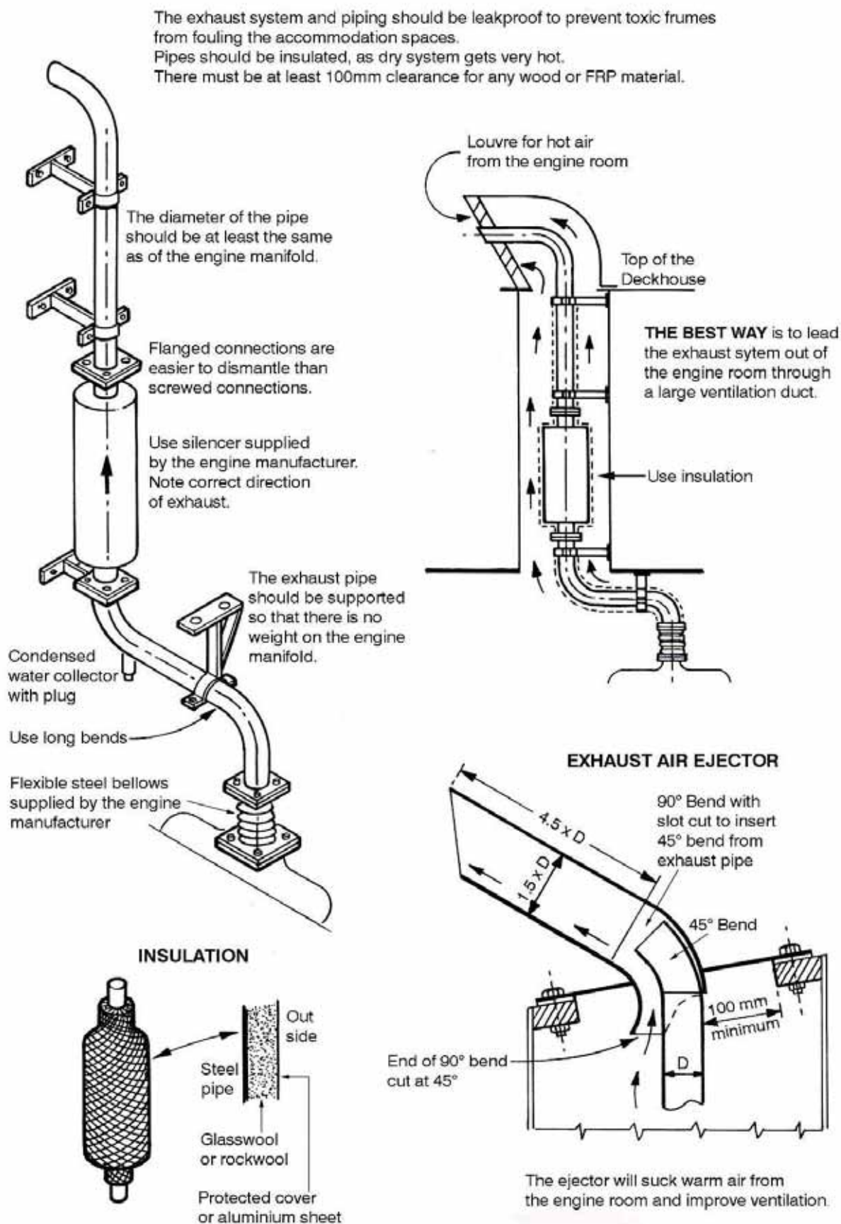
Figure 2.1 – Dry exhaust system – Sketches and notes
